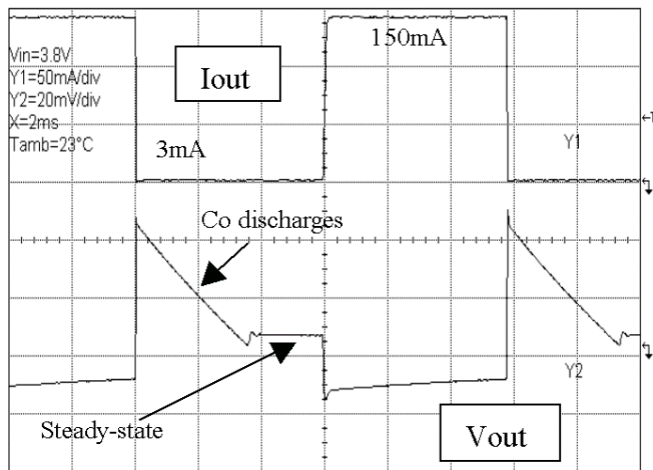
Figure 8. A Standard LDO Behavior when the Load Current Disappears
