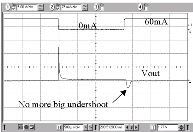
Figure 11. MC33761 with Load Transient Improvement
